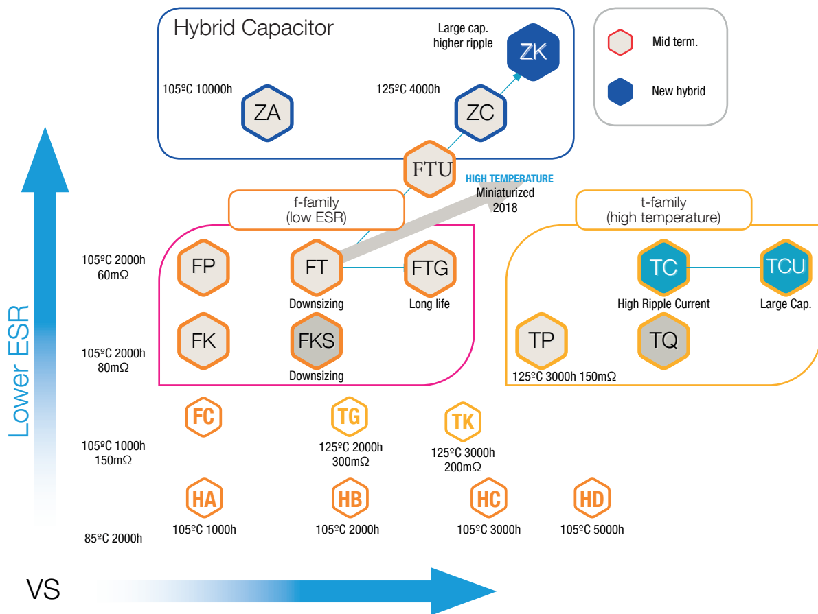
Figure 2 details the company's roadmap for smd technology electrolytic capacitors based on the demands of different applications
